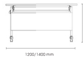
L1200*W450*H750/L1400*W450*H750 (mm)
