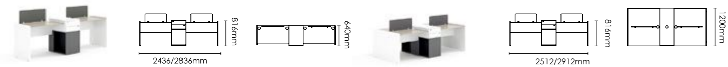
Single table with 2 seats FWY63.24 2436×640×816mm FWY63.28 2836×640×816mm
