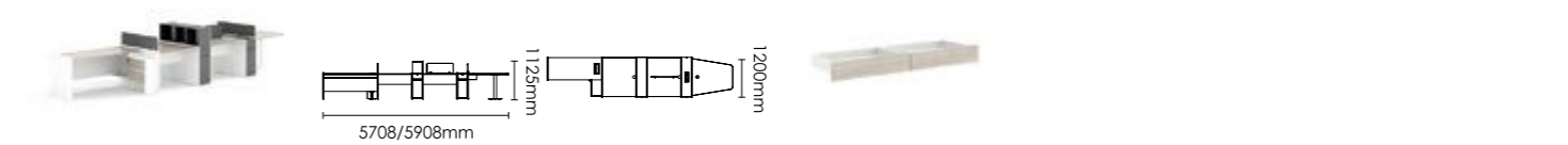
Workstation FWY50.57 5708×1200×1125mm FWY50.59 5908×1200×1125mm
