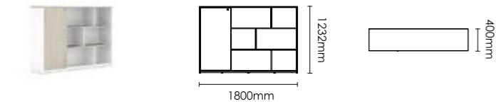
Main cabinet FWY90.18 1800×400×1232mm
