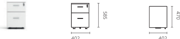
FKD32.04 402x470x585
