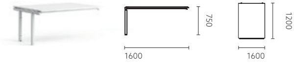
FKD73X.16MJ 1600x1200x750
