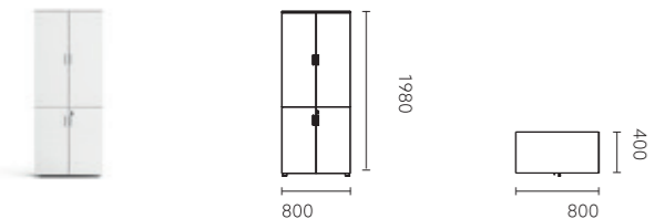
FKD91.08 800x400x1980
