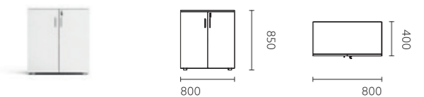
FKD31.08 800x400x850
