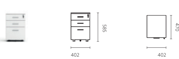
FKD33.04 402x470x585
