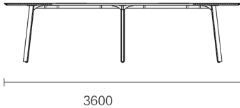
FNR72.30 3600 × 1200 × 750
