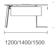
FNR66R.12/14/15 1200 × 600 × 750 / 1400 × 700 × 750 / 1500 × 700 × 750 FNR67.12/14/15 1200 × 1212 × 750 / 1400 × 1412 × 750 / 1500 × 1412 × 750
