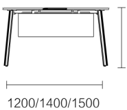
FNR60.12/14/15 1200 × 600 × 750 / 1400 × 700 × 750 / 1500 × 700 × 750 FNR62.12/14/15 1200 × 1212 × 750 / 1400 × 1412 × 750 / 1500 × 1412 × 750
