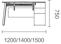
FNR64.12/14/15 1200 × 600 × 750 / 1400 × 700 × 750 / 1500 × 700 × 750 FNR65.12/14/15 1200 × 1212 × 750 / 1400 × 1412 × 750 / 1500 × 1412 × 750
