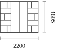
FNQ91.20 2200 × 400 × 1805
