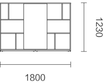
FNQ90.18 1800 × 400 × 1230
