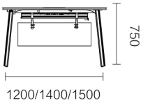
FNR60.12/14/15 1200 × 600 × 750 / 1400 × 700 × 750 / 1500 × 700 × 750 FNR62.12/14/15 1200 × 1212 × 750 / 1400 × 1412 × 750 / 1500 × 1412 × 750
