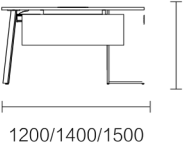
FNR64.12/14/15 1200 × 600 × 750 / 1400 × 700 × 750 / 1500 × 700 × 750 FNR65.12/14/15 1200 × 1212 × 750 / 1400 × 1412 × 750 / 1500 × 1412 × 750
