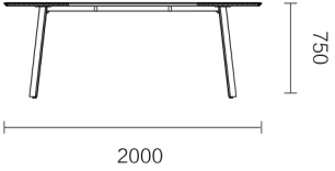
FNR70.20 2000 × 1000 × 750
