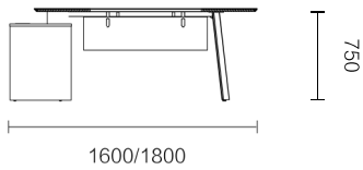
FNR80R.16/18/20 1600 × 1300 × 750 / 1800 × 1300 × 750/2000 × 1650 × 750
