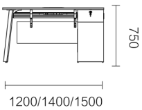
FNR66R.12/14/15 1200 × 600 × 750 / 1400 × 700 × 750 / 1500 × 700 × 750 FNR67.12/14/15 1200 × 1212 × 750 / 1400 × 1412 × 750 / 1500 × 1412 × 750
